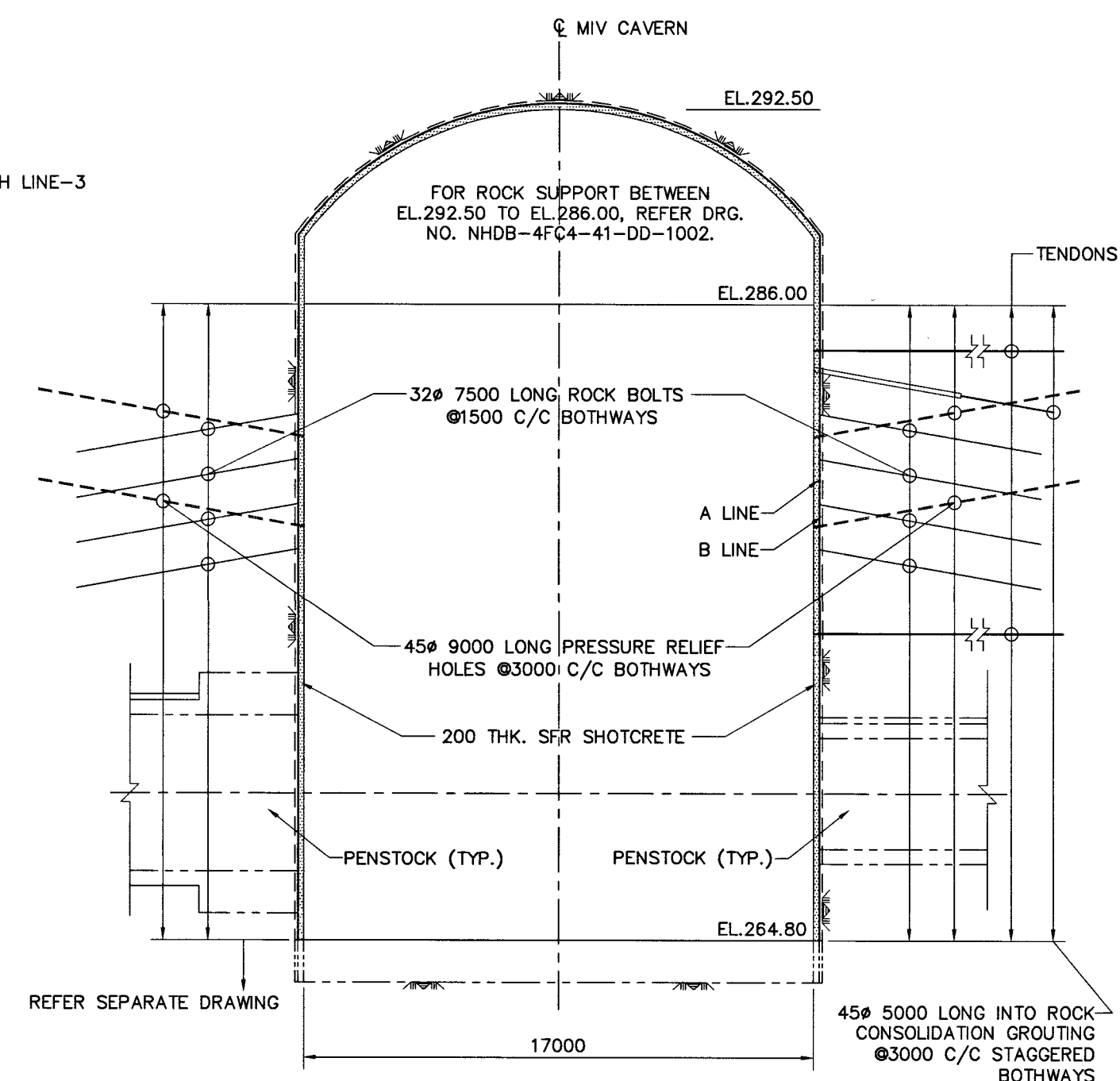
TYPICAL SECTION
