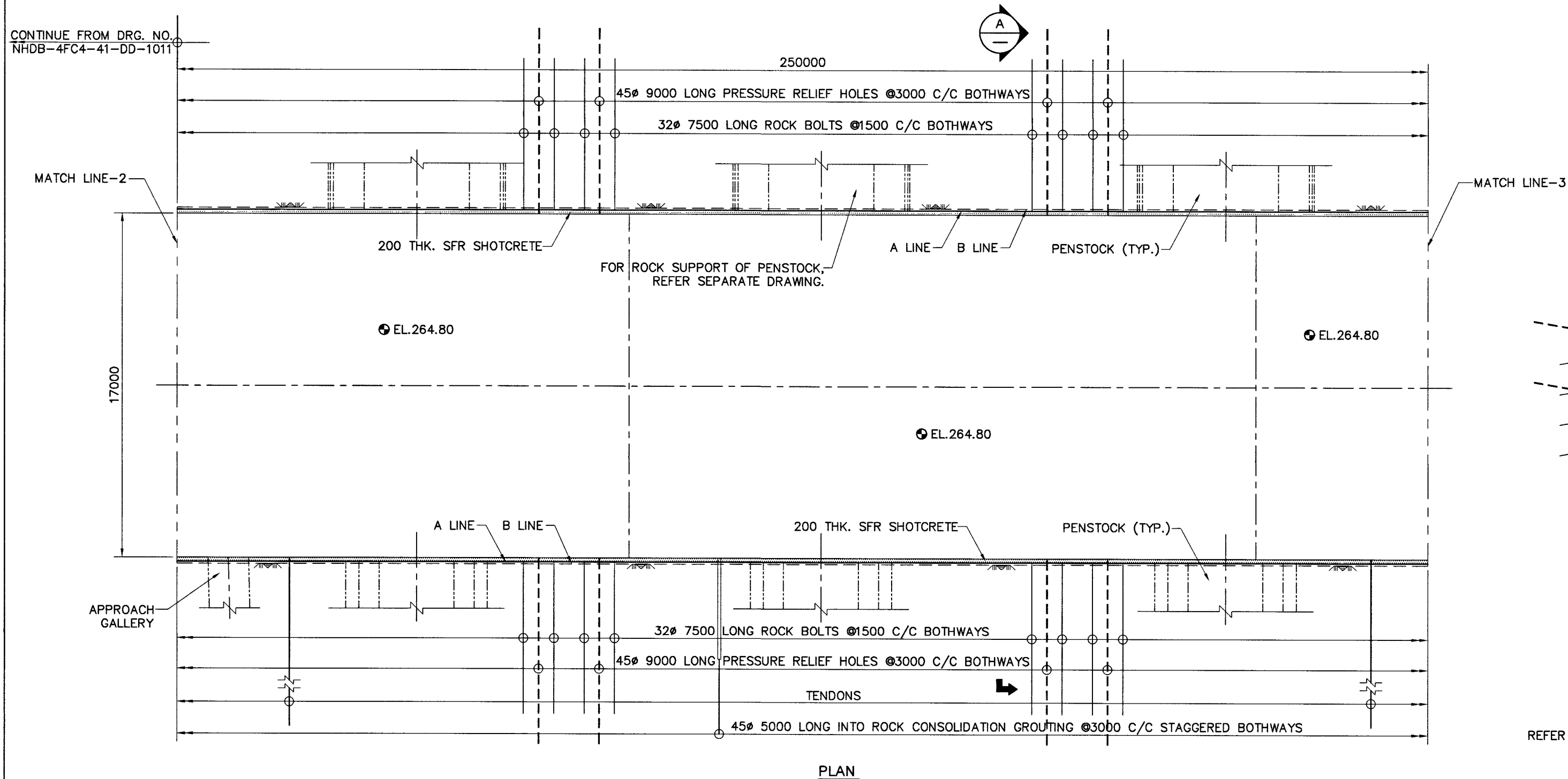
PLAN
